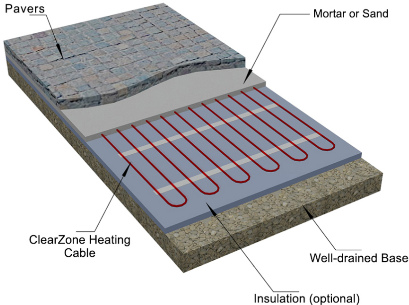
Illustration of ClearZone snow melting mats installed under stone pavers (with insulation).
