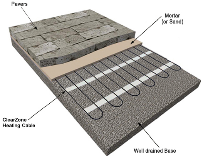
Illustration of ClearZone snow melting mats installed under stone pavers (without insulation).
