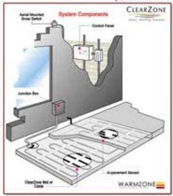
ClearZone snow melting system components.
