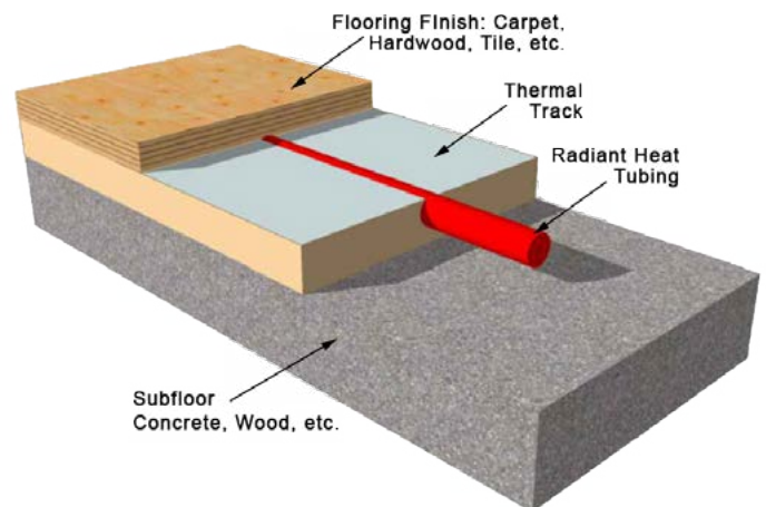
Example of a Hydronic Floor Heating System
