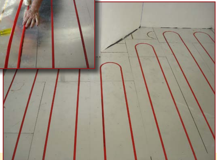
PEX tubing being installed in Raupanel for Warmzone hydronic floor heating system.
