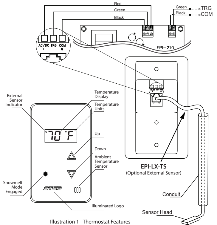
Illustration 1 - Thermostat Features
