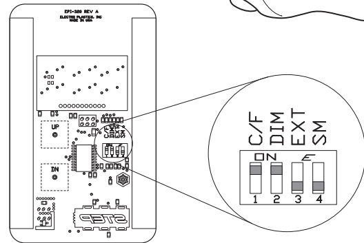
Illustration 3 - DIP Switches
