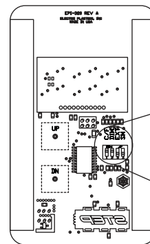
Illustration 3 - DIP Switches
