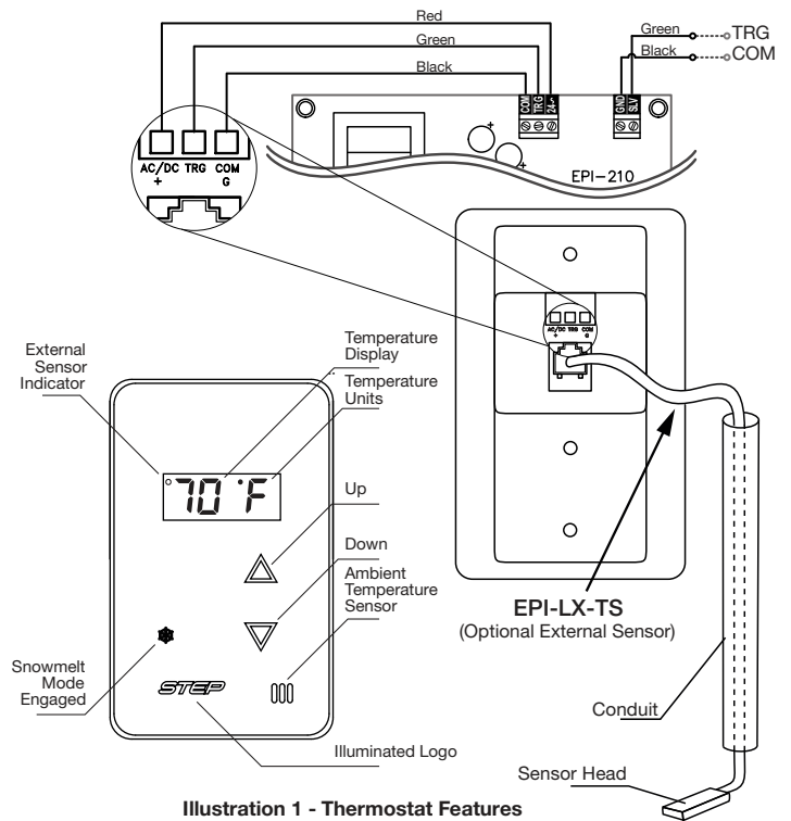
Illustration 1 - Thermostat Features
